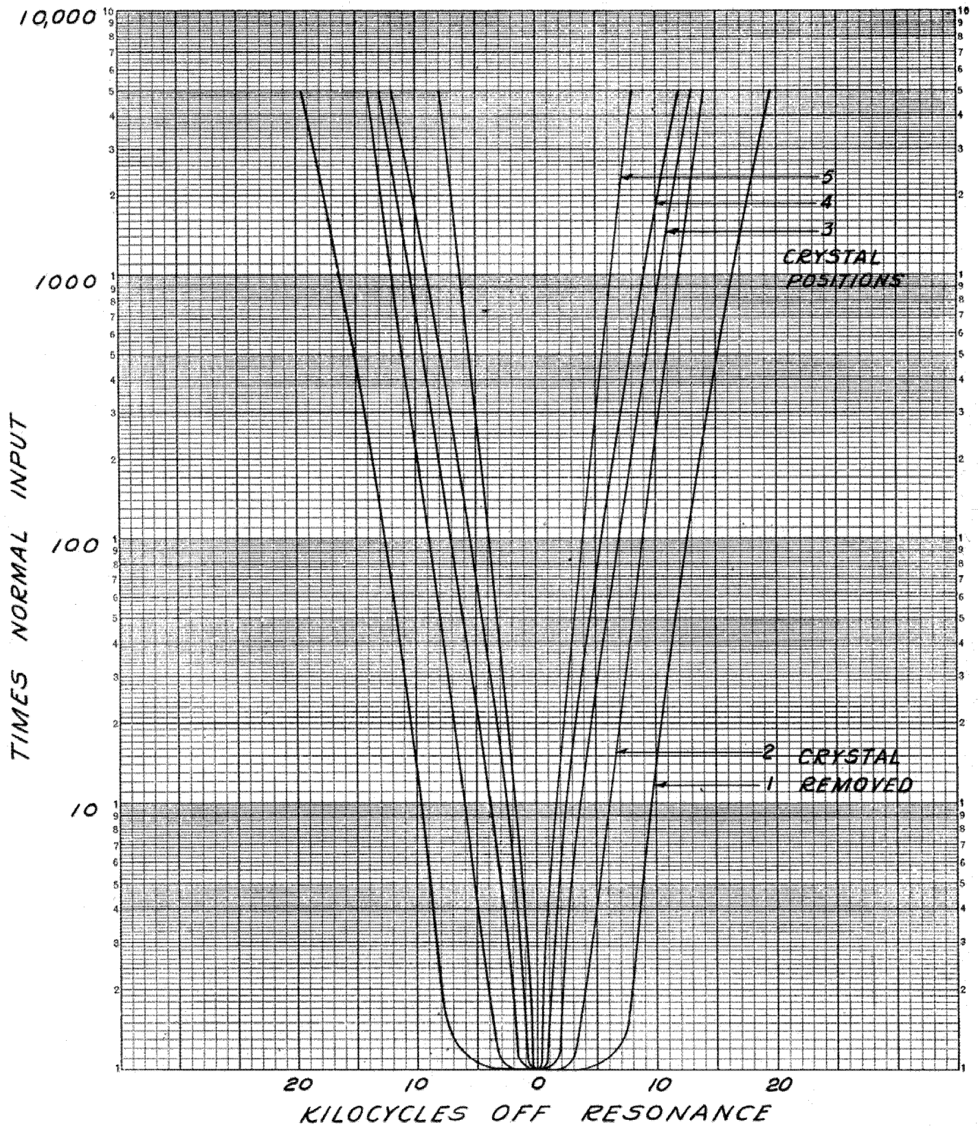
Figure 12.—General Purpose Communications Receiver—Selectivity Characteristics.
