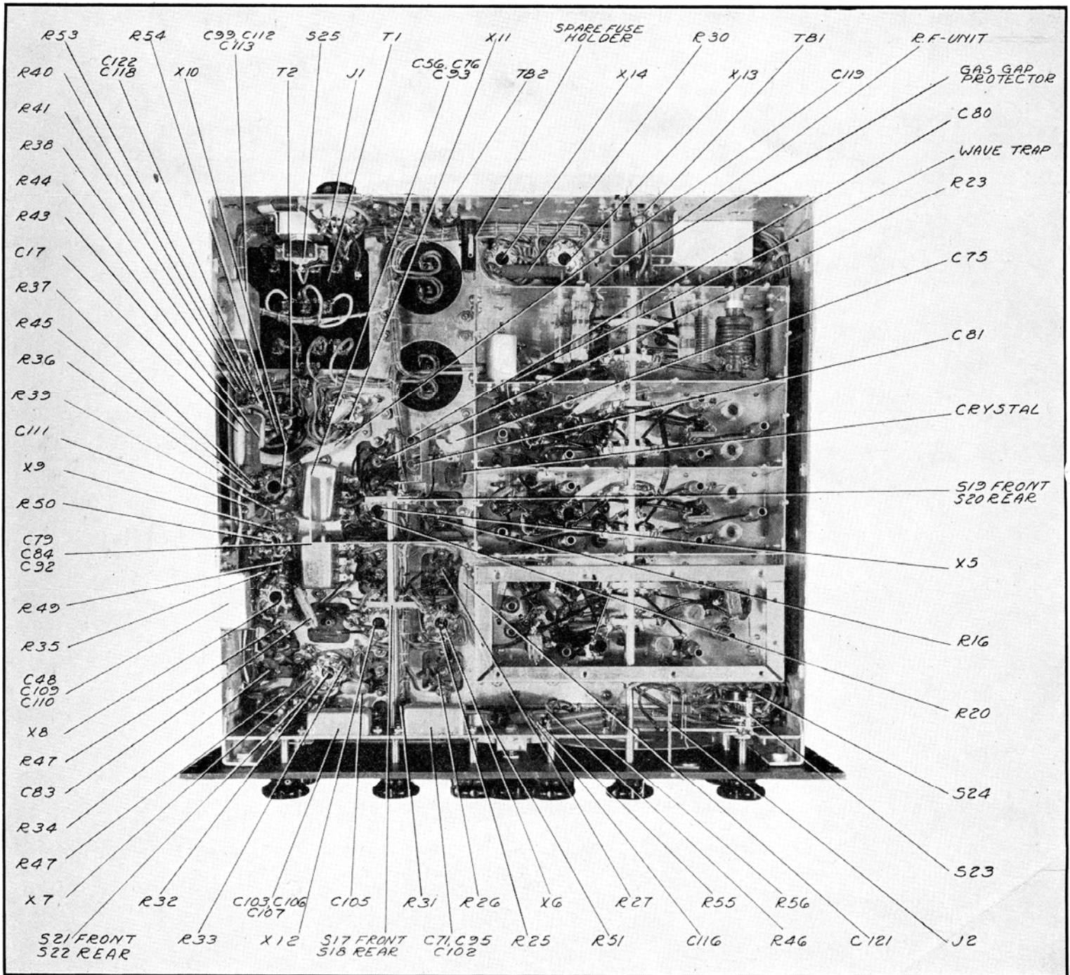
Figure 9.—General Purpose Communications Receiver—Bottom View—Covers Removed.
