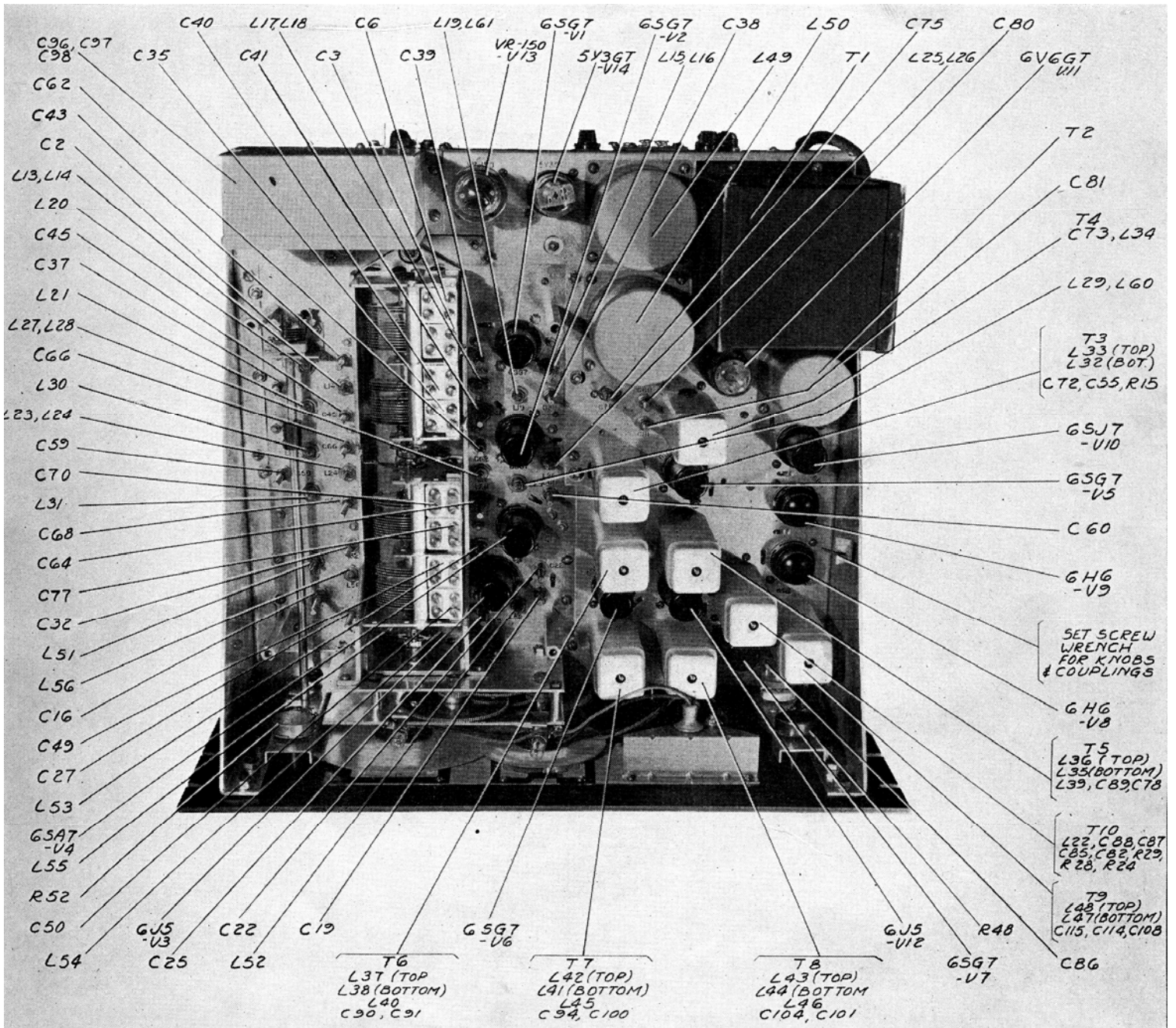
Figure 8.—General Purpose Communications Receiver—Top View—Covers Removed.
