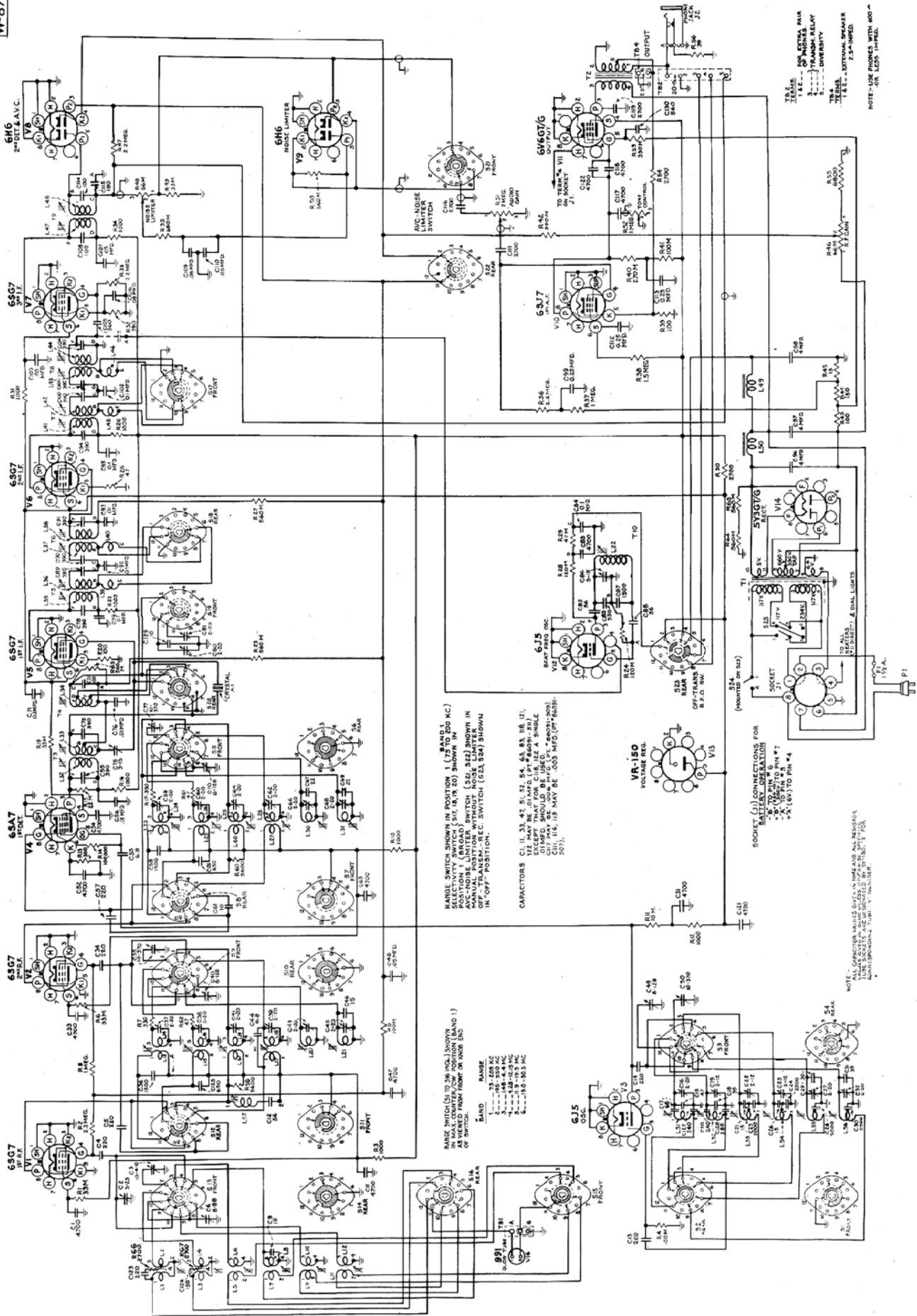
Figure 11.—General Purpose Communications Receiver—Schematic Diagram.
